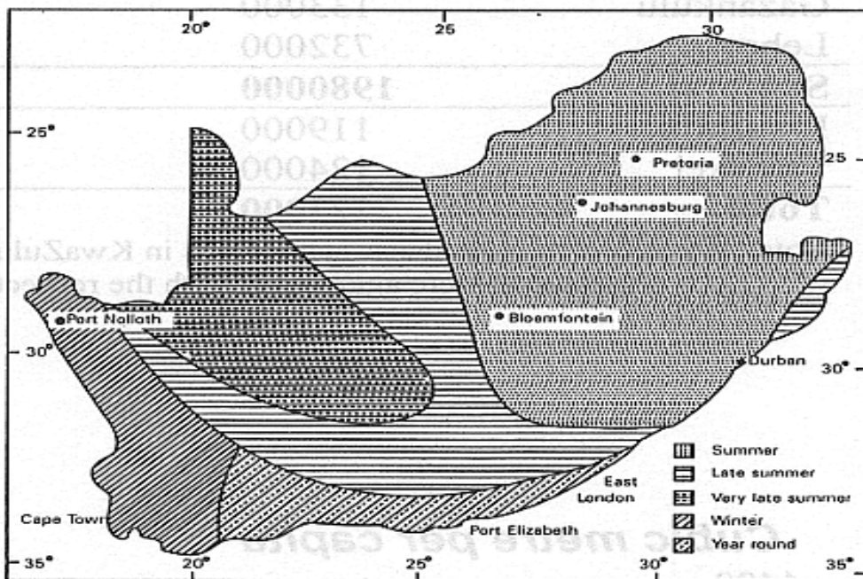
Fig. 3 Seasonal Rainfall Regions
