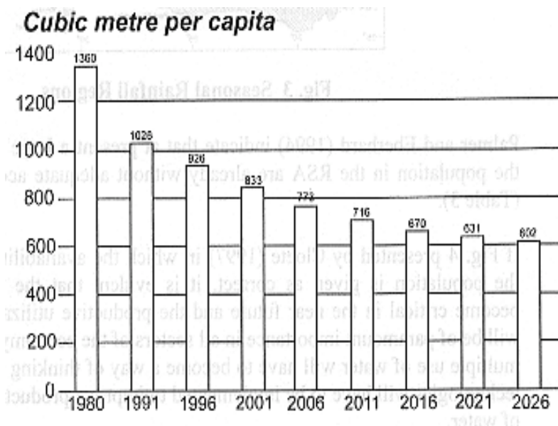
Fig. 4 Decrease in Availability of Water in the RSA
