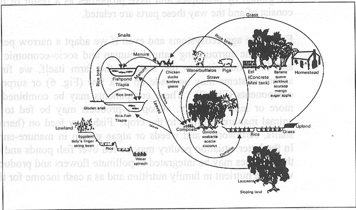
Fig. 7 Bio-resource Flow Model of an Integrated Agriculture – Aquaculture Farm.
