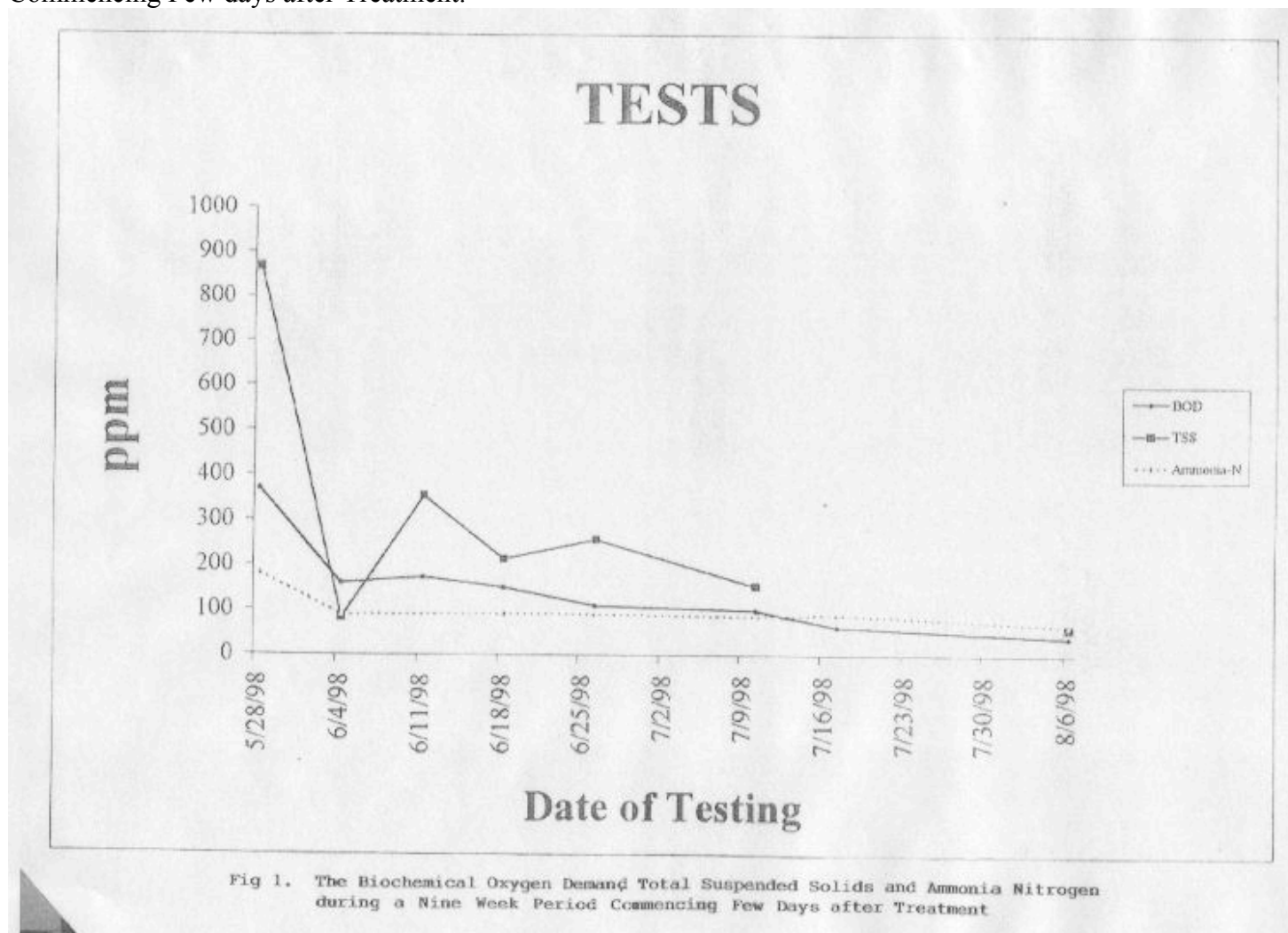
Fig 1. The Biological Oxygen Demand Total Suspended Solids and Ammonia Nitrogen during a Nine Week Period Commencing Few days after Treatment.
